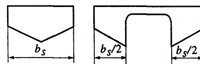
Fig 3.2.12 Breadth of Midship Slamming Reference Area
